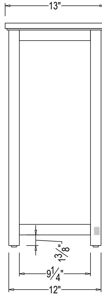
ANVA77WH DORSET STORAGE SIMPLE BASE
